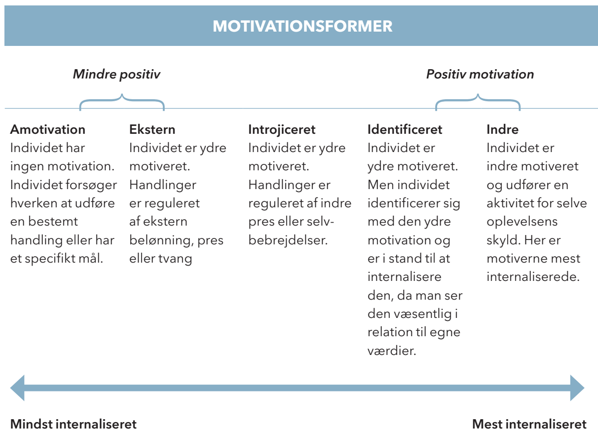
Figur 1. Motivation
